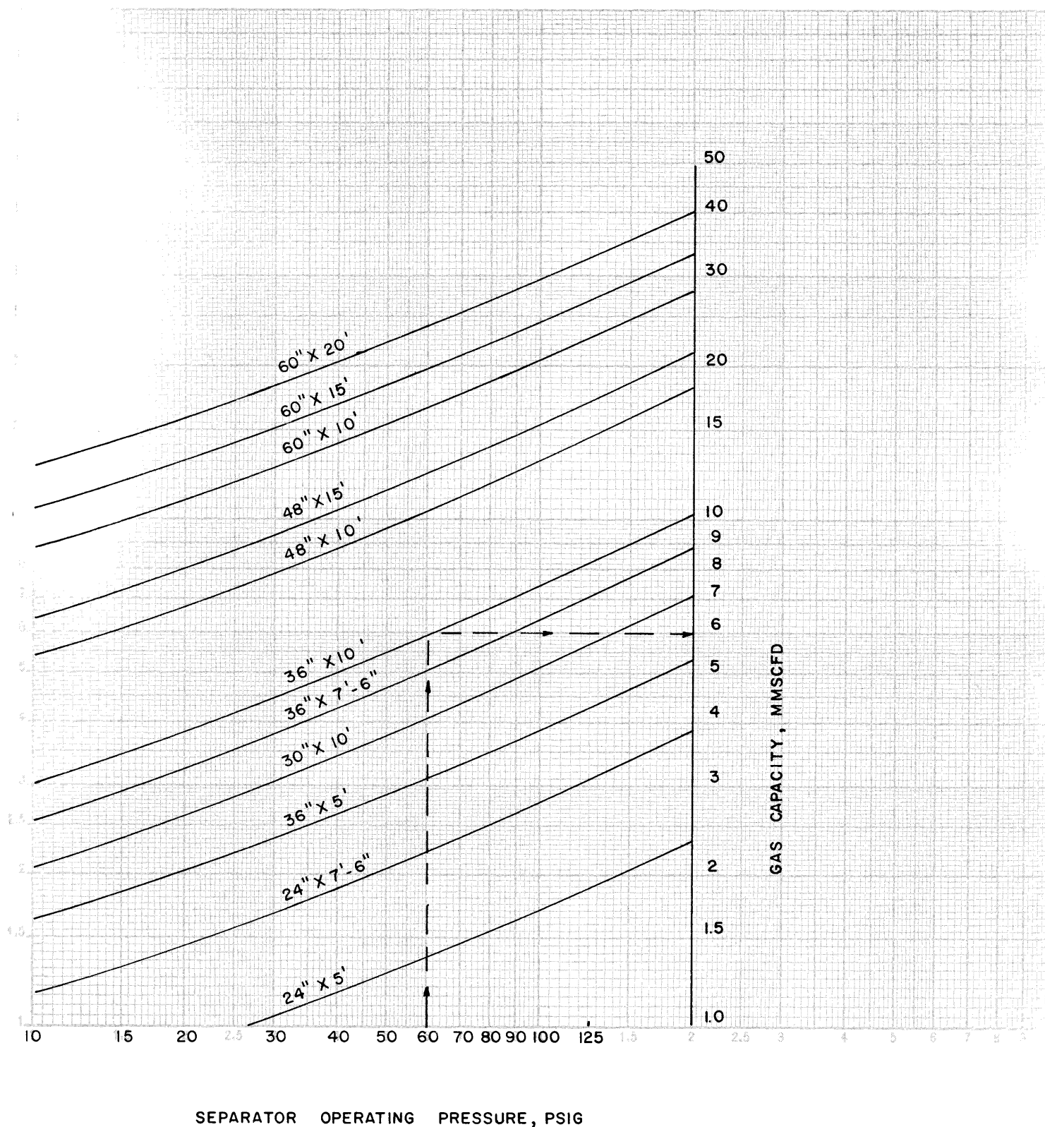
FIGURE 1 GAS CAPACITY OF VERTICAL L.P. SEPARATORS
