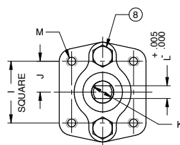
ACTUATOR MOUNTING
