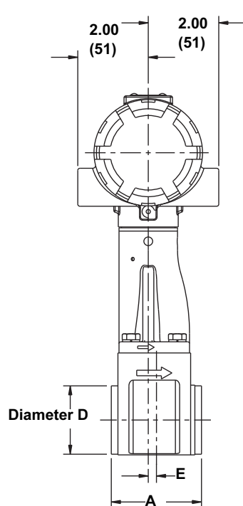
FIGURE 4. Wafer-Style Dimensional Drawings ( \frac{1}{2} -through 8 in./15 through 200 mm Line Sizes)
