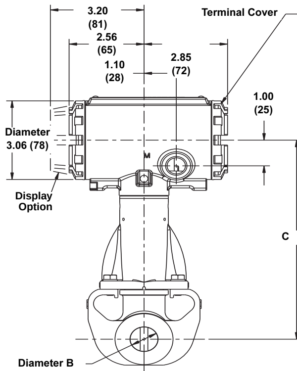
FIGURE 4. Wafer-Style Dimensional Drawings ( \frac{1}{2} -through 8 in./15 through 200 mm Line Sizes)
