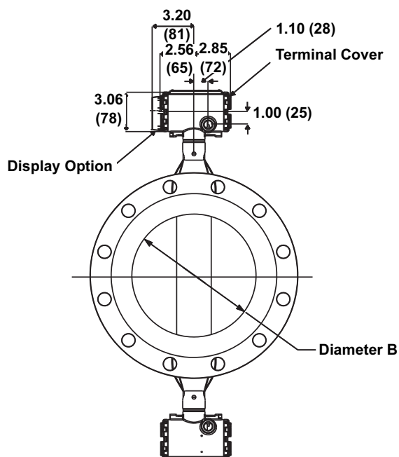
FIGURE 6. Vortex Dual-Sensor Style Flowmeter Dimensional Drawings (6 - 8 in (150 - 200mm) with 900# or 1500# flanges and all 10 - 12 in. (250-300mm) line sizes)
