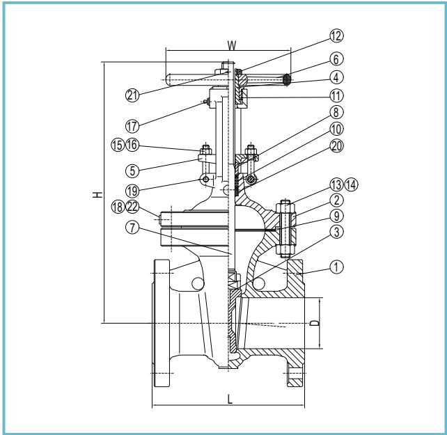
Flanged, ASME CLASS 300 (PN50, DN50~200) Integral Seat; flexible wedge(solid wedge only for DN50); Optional Stellite Seat Face
