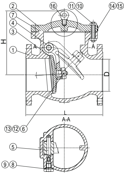
Flanged, ASME CLASS 150~300 (PN20-50) Integral Seat; Optional Stellite Seat Face
